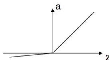
Leaky ReLU
