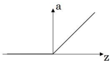
ReLU
