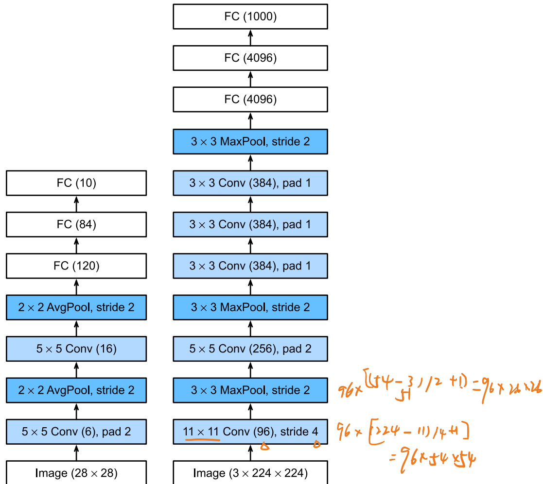
图6.1.2: 从LeNet (左) 到AlexNet (right)
