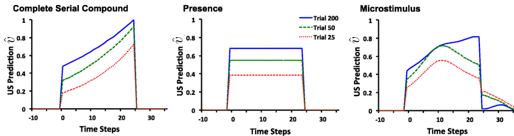
Figure 14.6: Time course of US prediction over the course of acquisition for the TD model with three different stimulus representations. Left: With the complete serial compound (CSC), the US prediction increases exponentially through the interval, peaking at the time of the US. At asymptote (trial 200), the US prediction peaks at the US intensity (1 in these simulations). Middle: With the presence representation, the US prediction converges to an almost constant level. This constant level is determined by the US intensity and the length of the CS–US interval. Right: With the microstimulus representation, at asymptote, the TD model approximates the exponentially increasing time course depicted with the CSC through a linear combination of the different microstimuli. Adapted with minor changes from Learning & Behavior , Evaluating the TD Model of Classical Conditioning, volume 40, 2012, E. A. Ludvig, R. S. Sutton, E. J. Kehoe. With permission of Springer.
